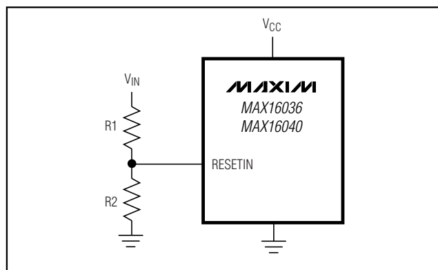
Figure 4. Setting RESETIN Voltage for the MAX16036/MAX16040
