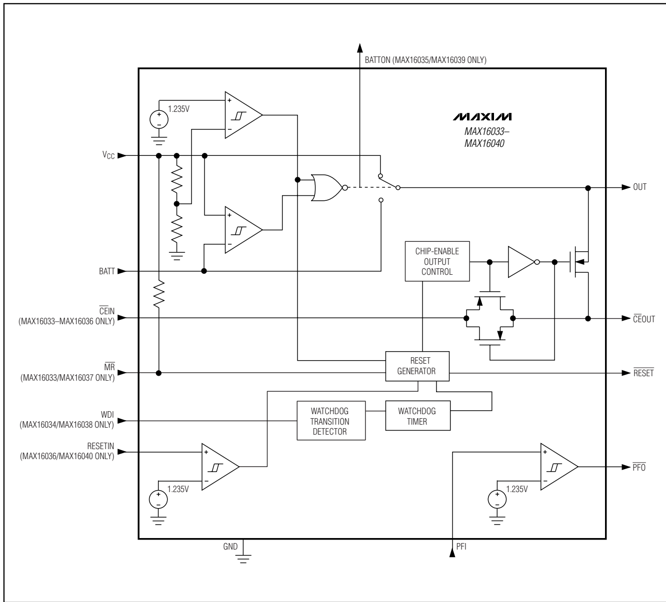
Functional Diagram
