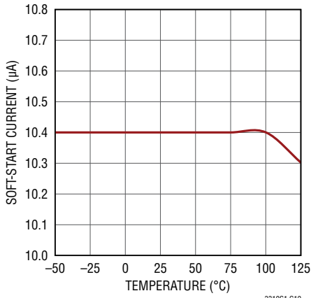
Soft-Start Current
