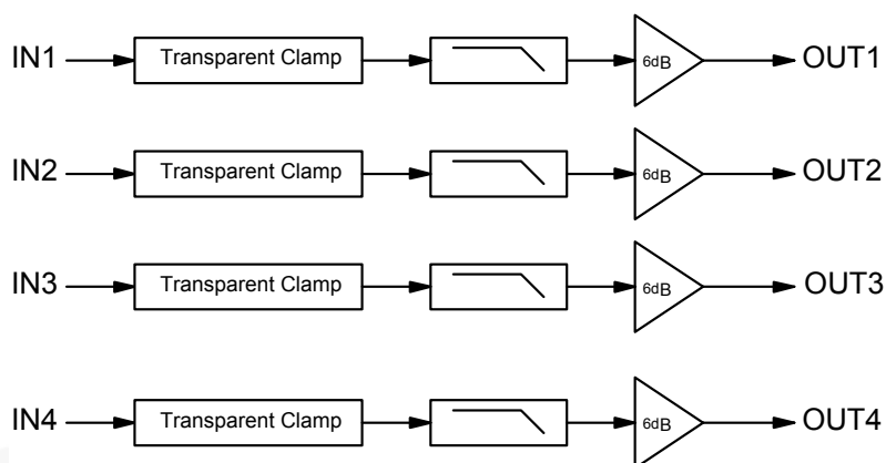
Figure 1. Block Diagram
