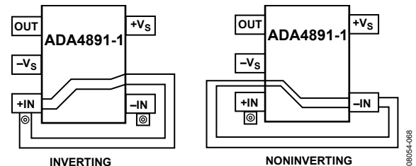
Figure 67. Guard Ring Layout, 5-Lead SOT-23
