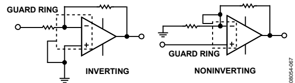
Figure 66. Guard Ring Configurations
