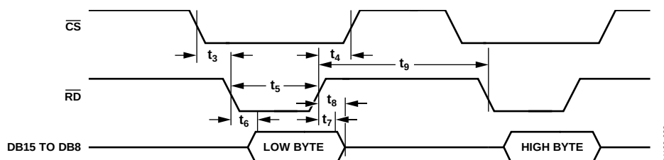
Figure 26. Parallel Interface—Read Cycle for Byte Mode of Operation ( \overline{\text{W}}/\text{B} = 1 , HBEN = 0)
