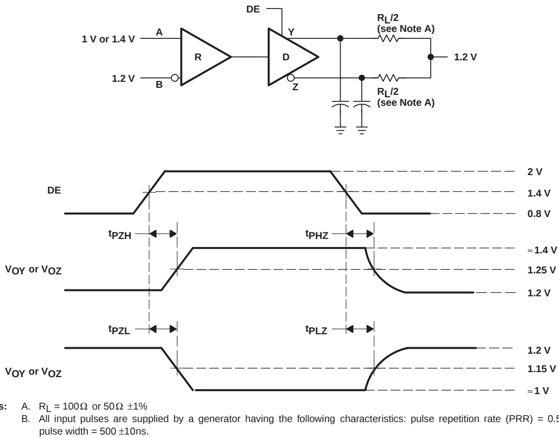
Figure 6. Enable and Disable Timing Circuit
