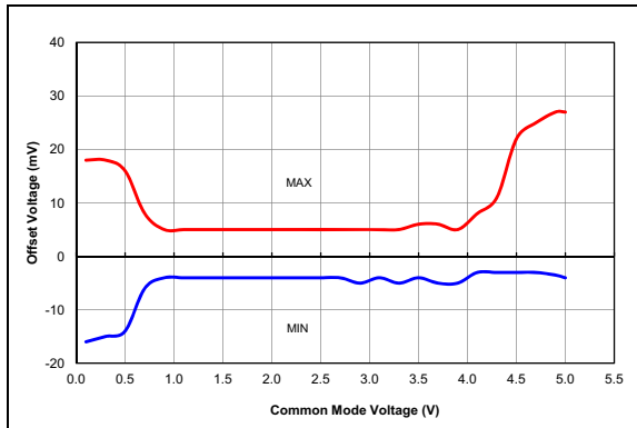
FIGURE 38-55: Comparator Offset, NP Mode ( CxSP = 1 ), V_{DD} = 5.5V , Typical Measured Values from -40^\circ C to 125^\circ C , PIC16F18857/77 Only.
