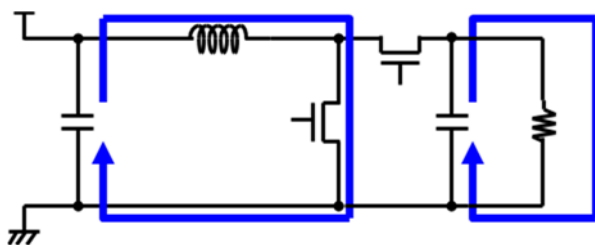
NMOSFET-ON (BOOST)
