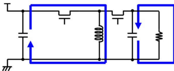
PMOSFET-ON (INVERTING)
