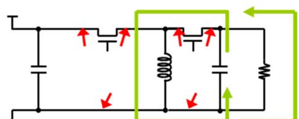
NMOSFET-ON (INVERTING)
