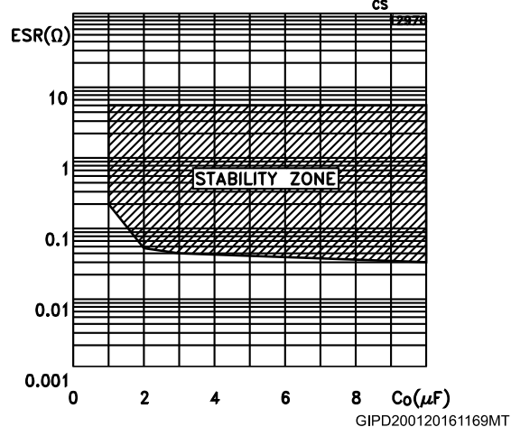
Figure 19: Worst case: lowest output version
