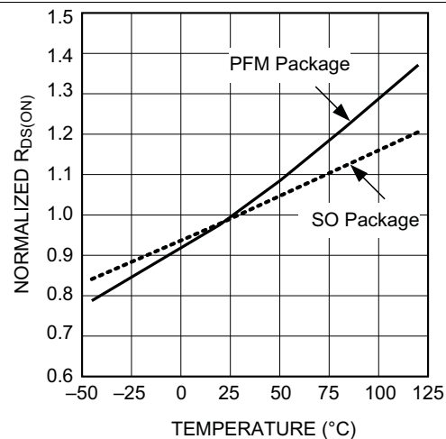
Figure 6. Normalized R_{DS(ON)} vs Temperature
