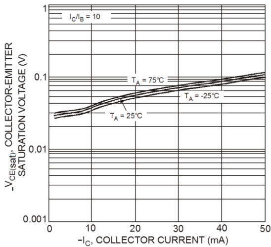
Fig. 24 Typical V_{CE(sat)} vs. I_C
