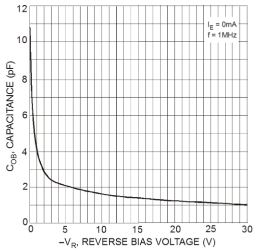
Fig. 4 Typical Output Capacitance
