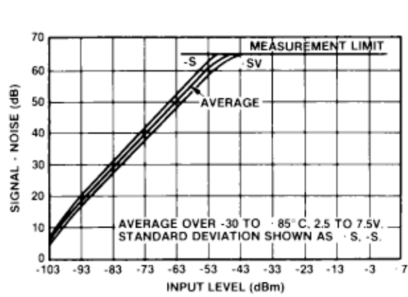
Fig. 14 Signal + noise to noise ratio vs input level
