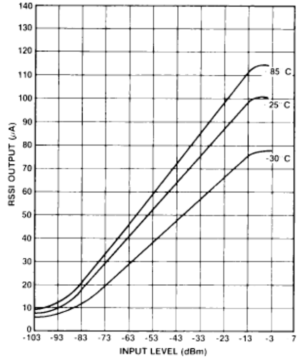
Fig. 11 RSSI output vs input level and temperature ( V_{\text{CC}} = 2.5\text{V} )
