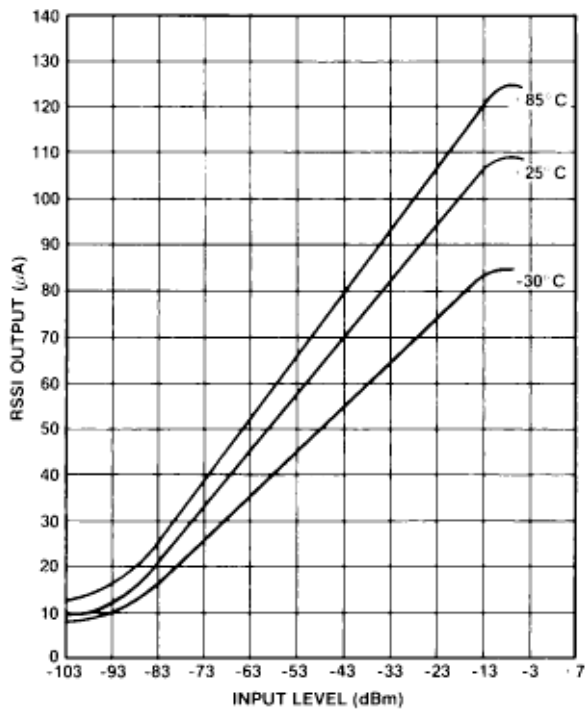
Fig. 12 RSSI output vs input level and temperature ( T_{\text{CC}} = 5\text{V} )
