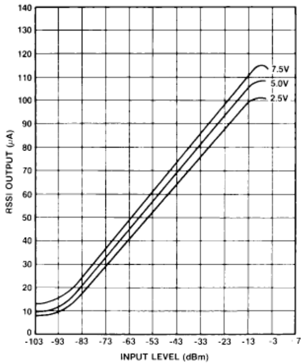
Fig. 10 RSSI output vs input and supply voltage ( T_{\text{amb}} = 20^\circ\text{C} )
