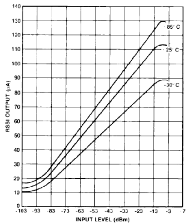
Fig. 13 RSSI output vs input level and temperature ( V_{\text{CC}} = 7.5\text{V} )
