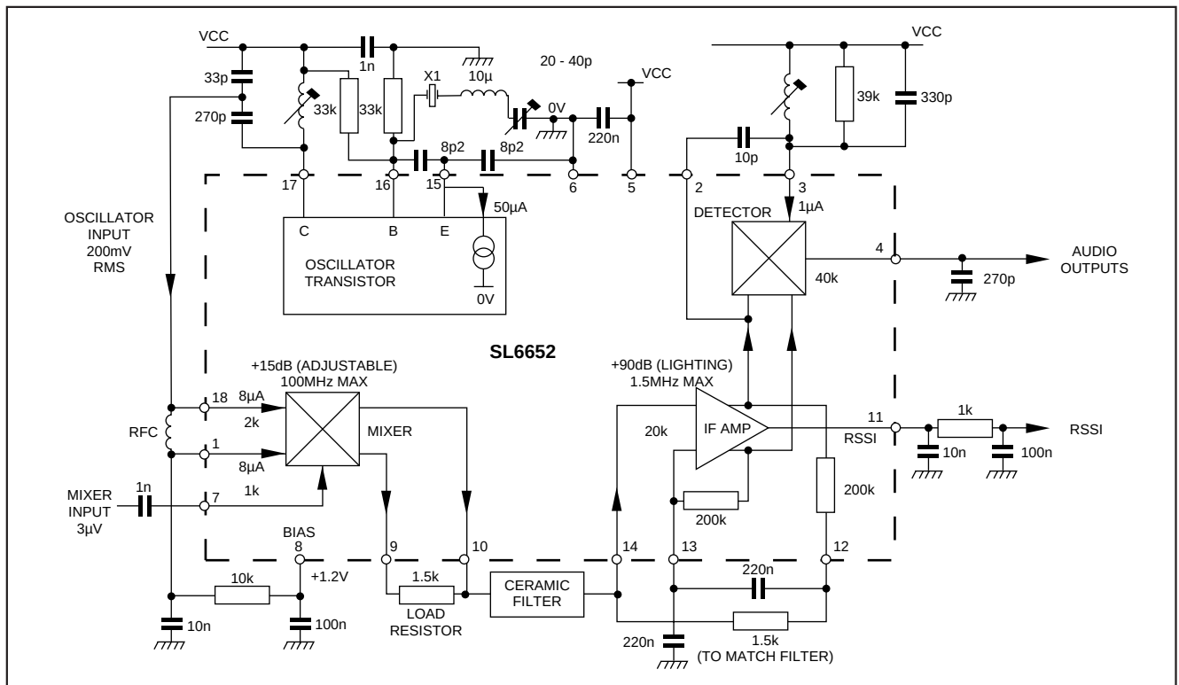
Fig. 2 block diagram
