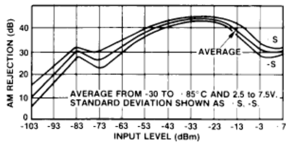
Fig. 9 AM rejection and input level
