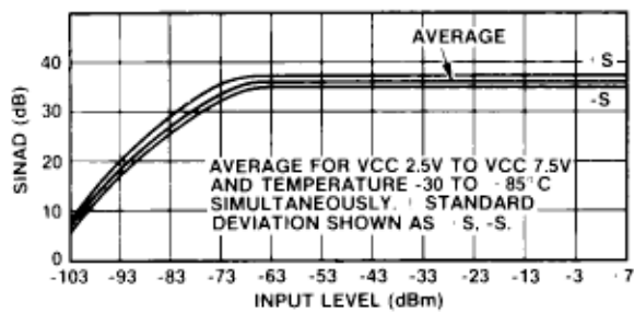
Fig. 8 SINAD and input level
