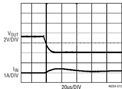
Short-Circuit with No Load Current Applied
