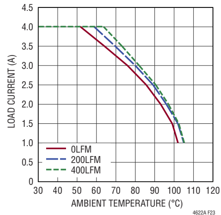
Figure 23. 16V Input to 12V Output Derating Curve, No Heat Sink
