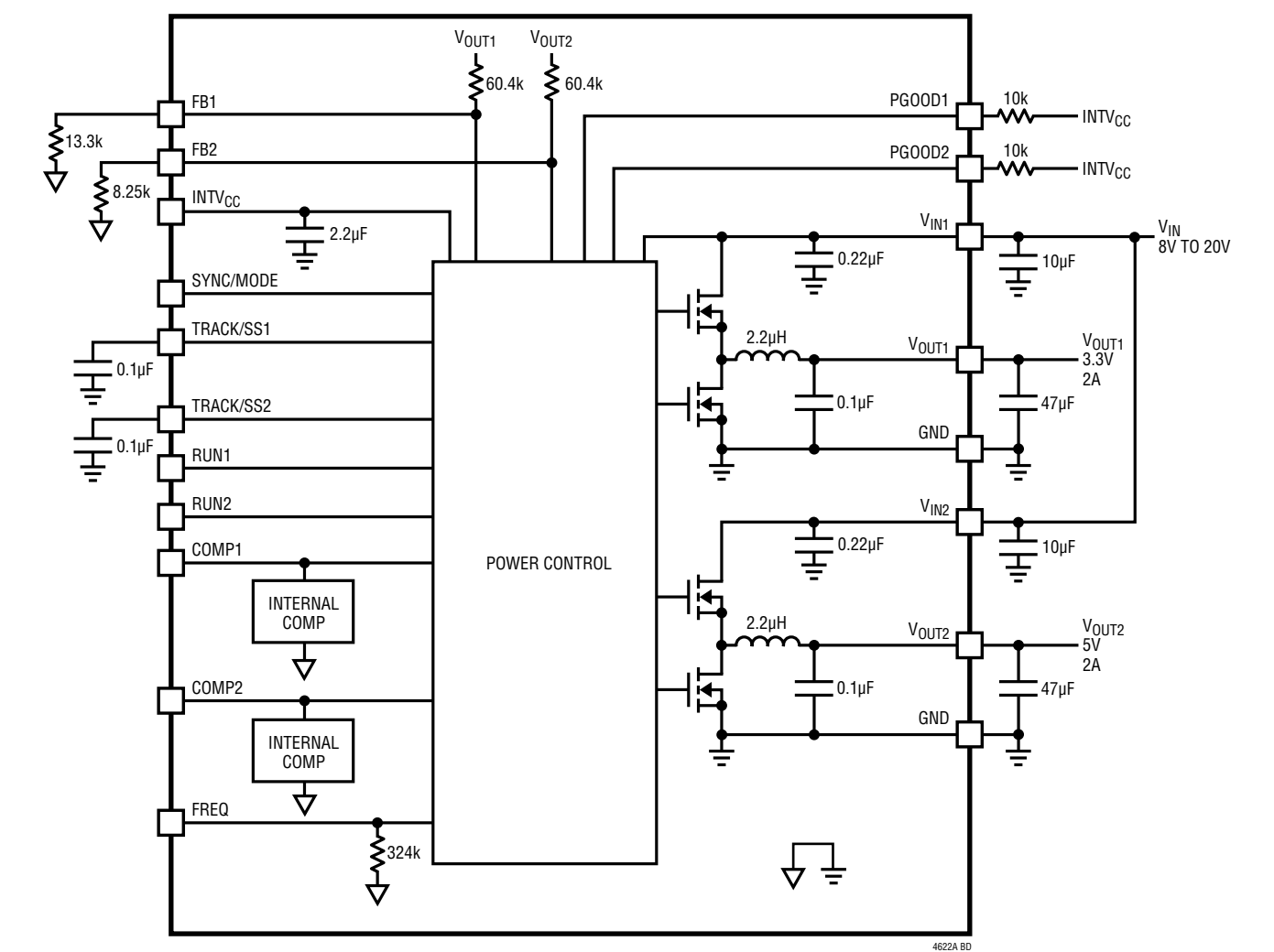
Figure 1. Simplified LTM4622A Block Diagram
