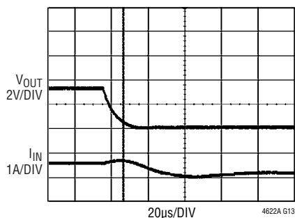
Short-Circuit with 2A Load Current Applied
