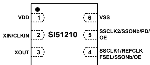
Figure 6.1. 6-Pin TDFN
