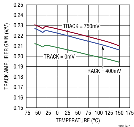
TRACK Amplifier Gain
