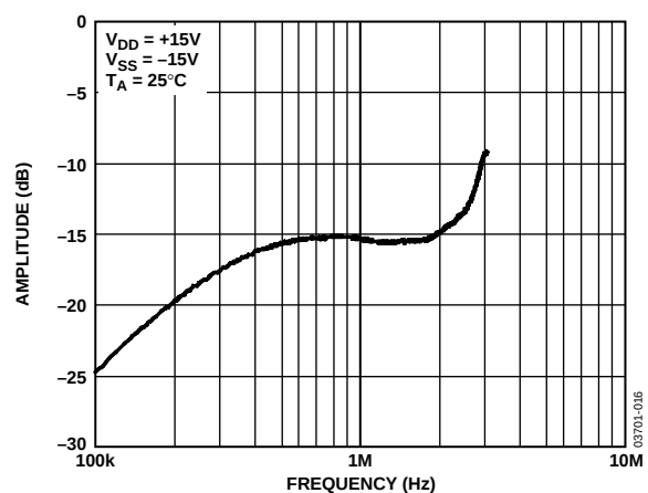
Figure 16. Force Amplifier AC PSRR, Mode 3, C_{\text{COMP}} = 100\text{pF}
