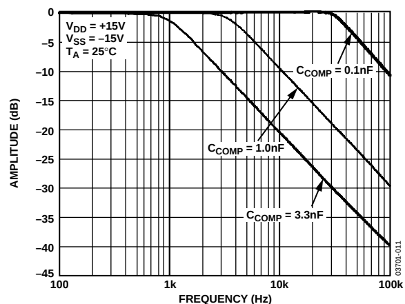
Figure 11. Force Amplifier Bandwidth, Mode 2 (400 \mu\text{A} )
