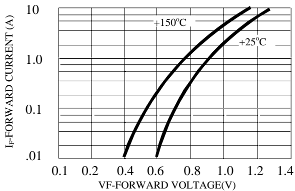
Fig. 4-TYPICAL FORWARD CHARACTERISTICS
