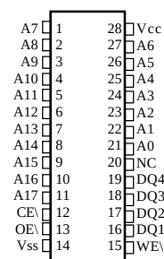
28-Pin DIP (C) (400 MIL)
