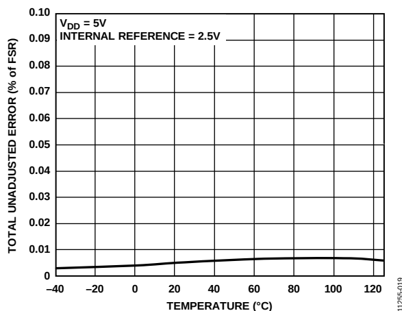
Figure 19. Total Unadjusted Error (TUE) vs. Temperature
