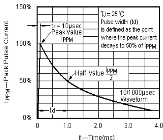
Fig. 3--Pulse Waveform
