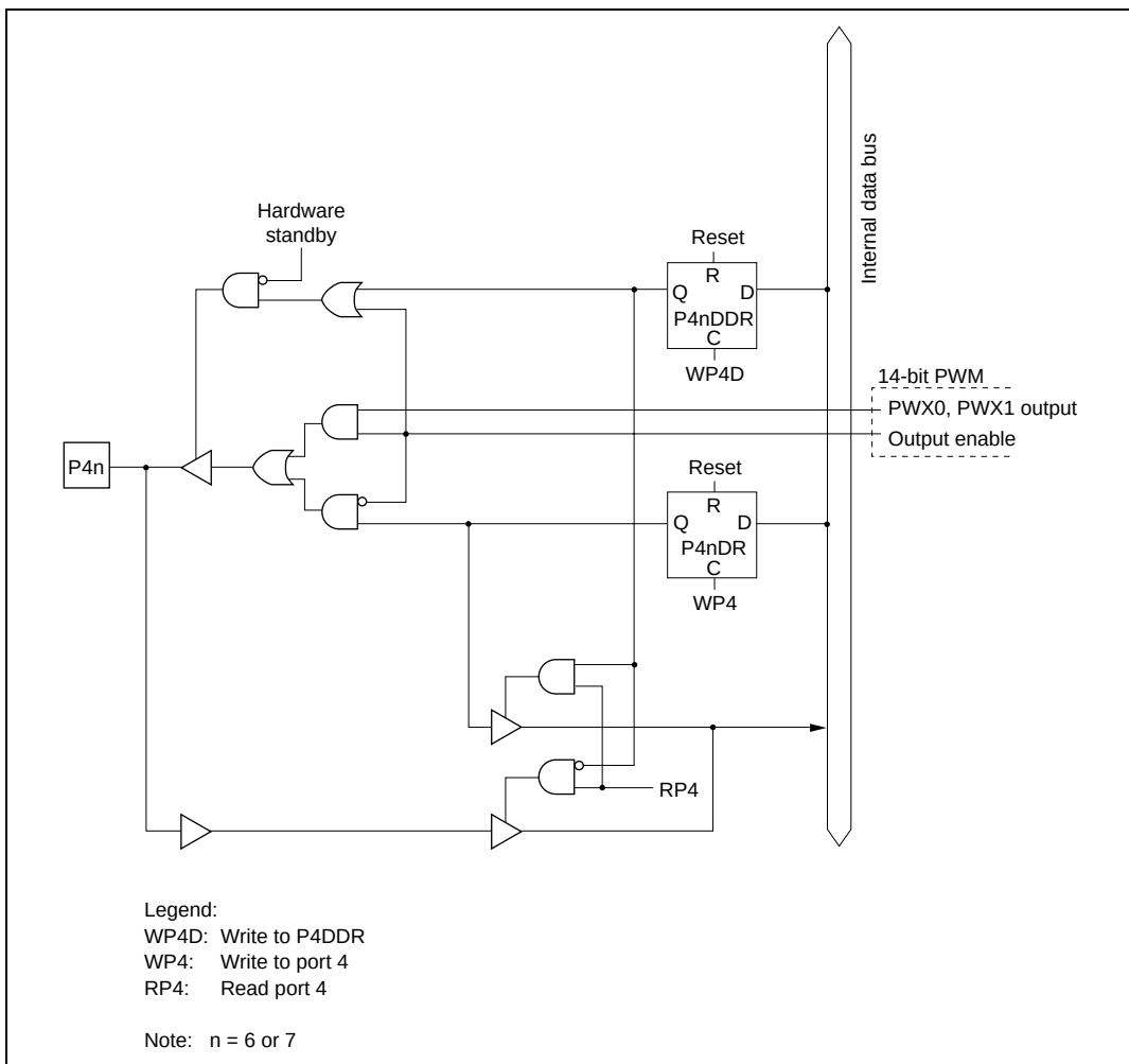
Figure C.12 Port 4 Block Diagram (Pins P46, P47)
