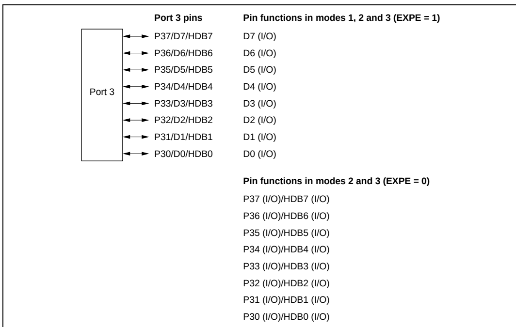
Figure 8.9 Port 3 Pin Functions
