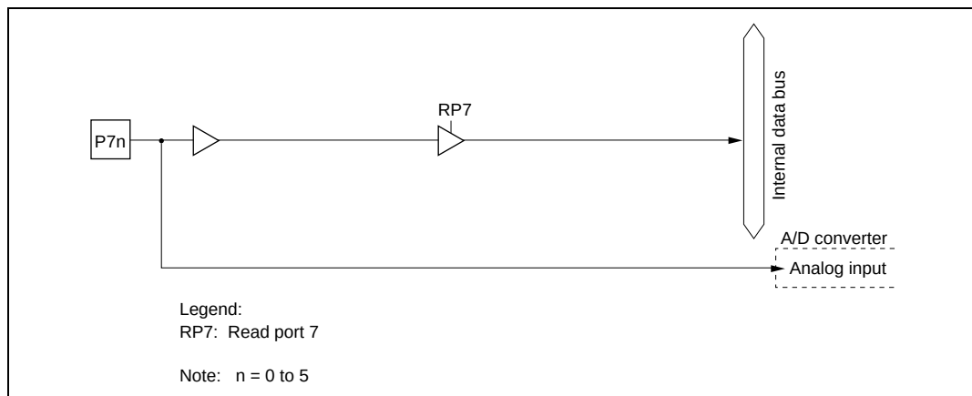
Figure C.21 Port 7 Block Diagram (Pins P70 to P75)
