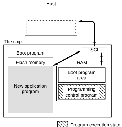
Figure 22.4 Boot Mode
