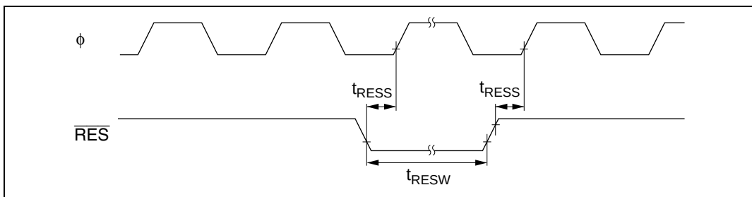
Figure 25.8 Reset Input Timing
