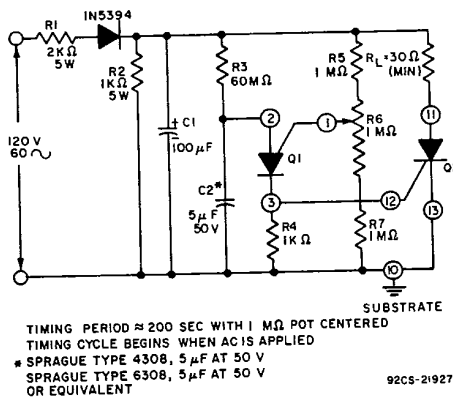
Fig. 27 — AC line-operated one-shot timer.
