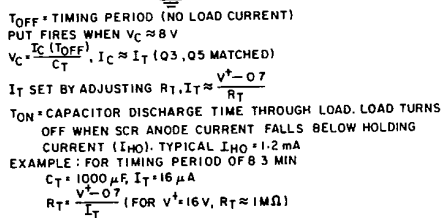
Fig.34 — Low-current-drain battery-operated long interval astable timer.
