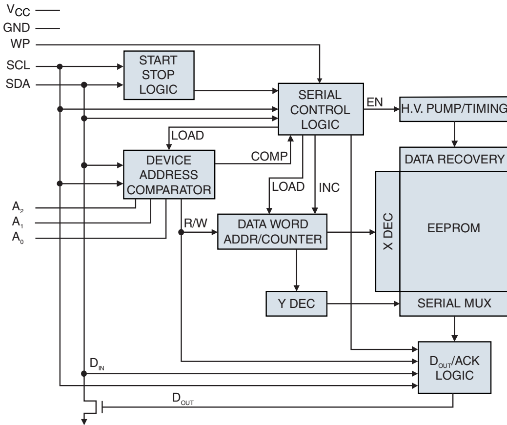
Figure 1. Block Diagram
