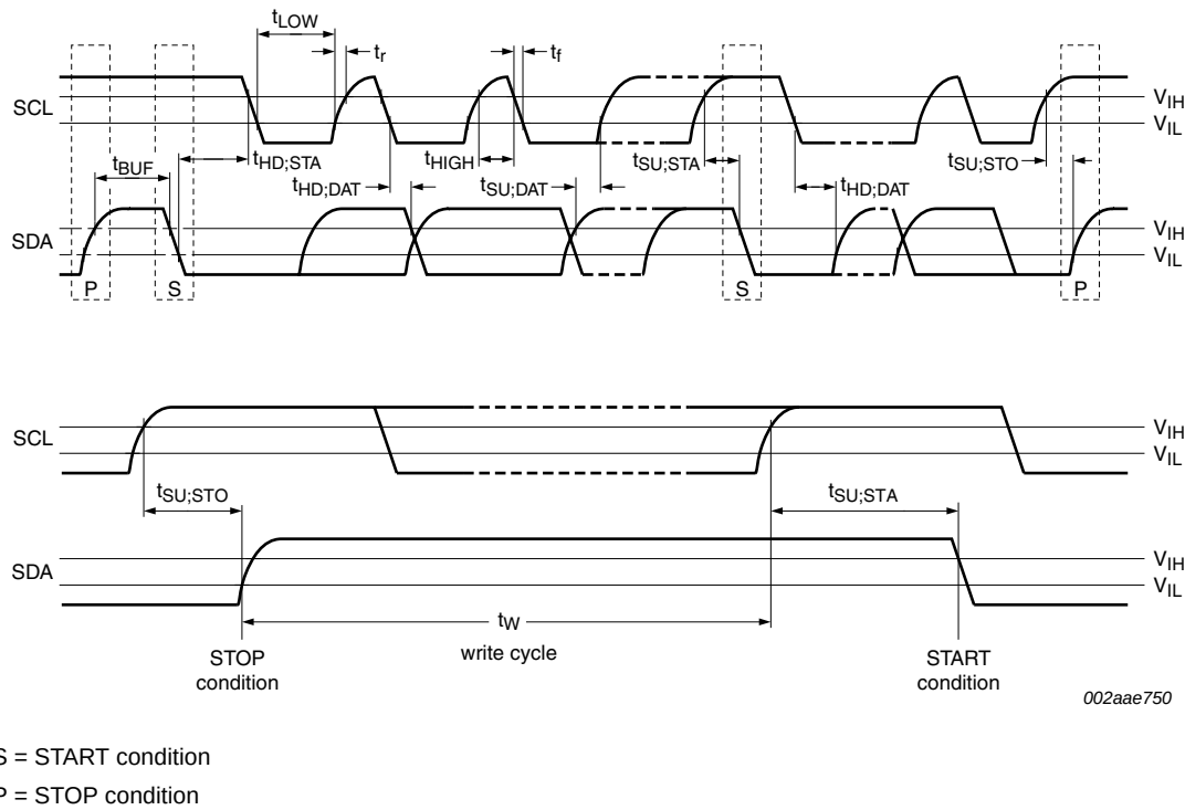
Fig 40. AC waveforms
