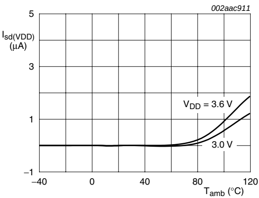
Fig 27. Shutdown supply current
