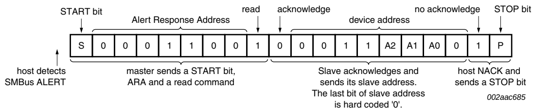
Fig 9. How SE97 responds to SMBus ALERT Response Address
