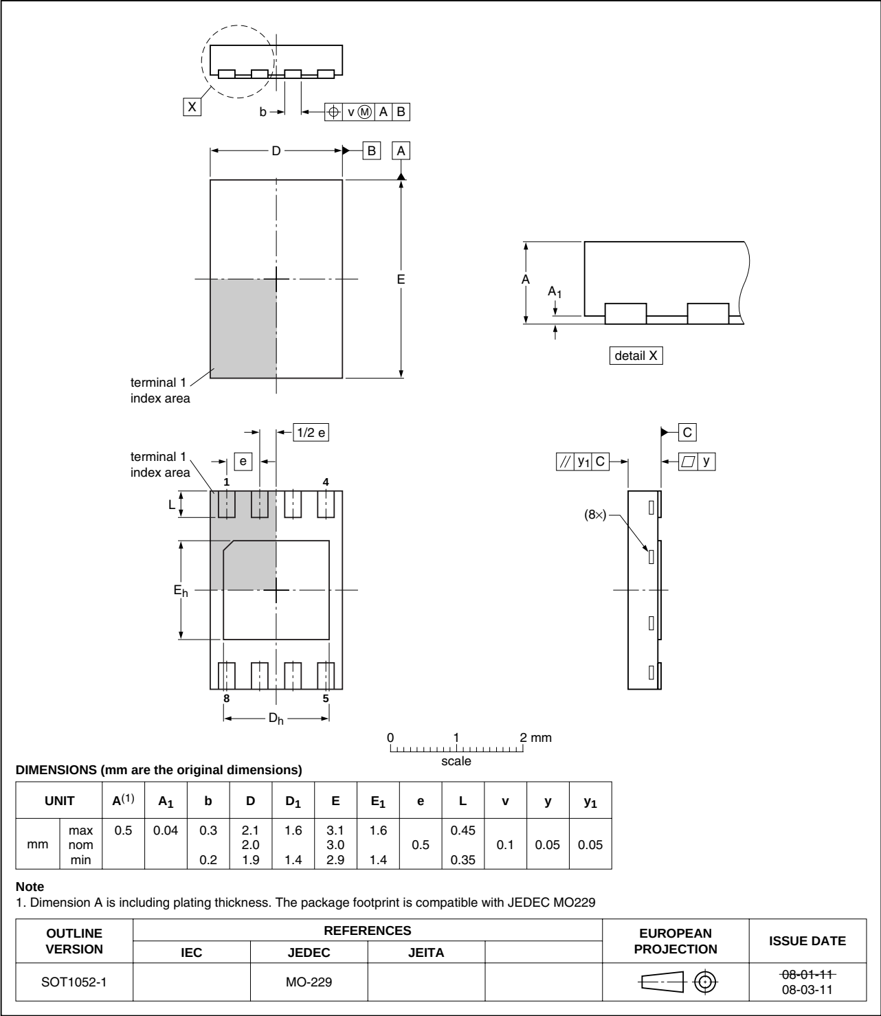
Fig 43. Package outline SOT1052-1 (HXSON8)
