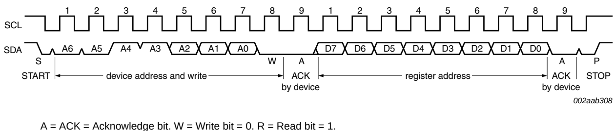
Fig 10. SMBus/I 2 C-bus write to the Pointer register
