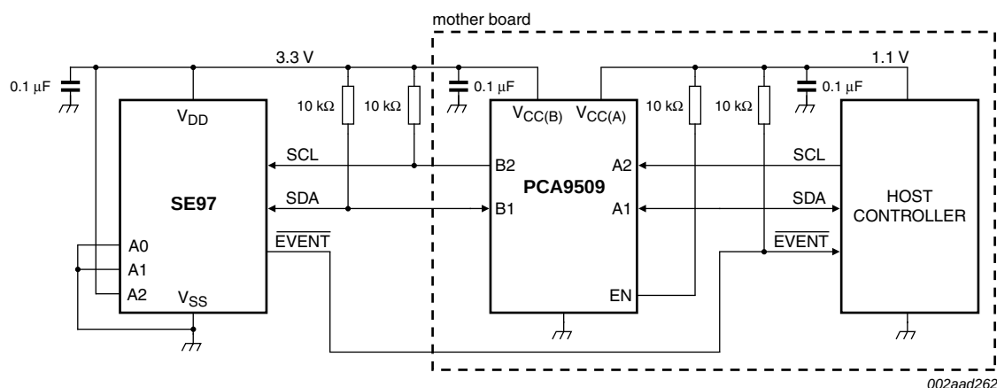
Fig 24. SE97 interfacing with 1.1 V host controller
