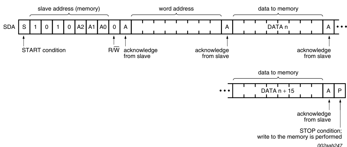
Fig 16. Page Write timing
