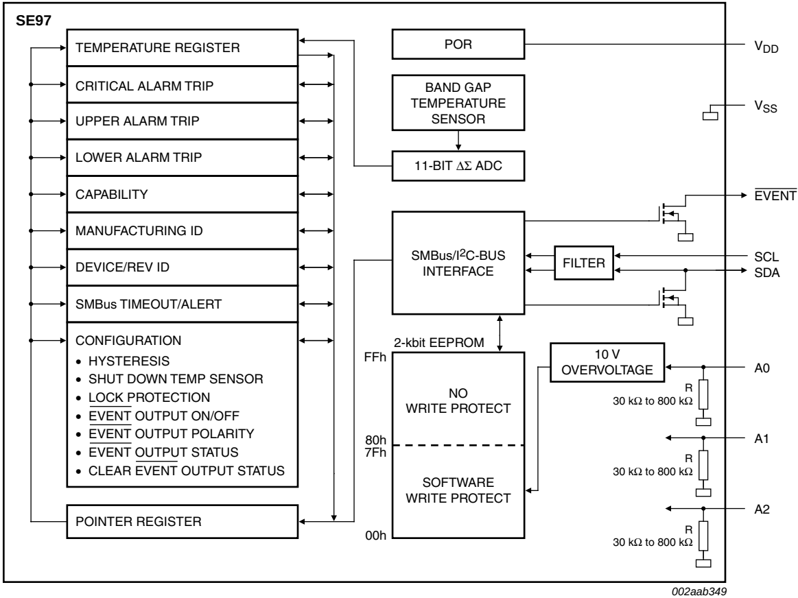
Fig 1. Block diagram of SE97
