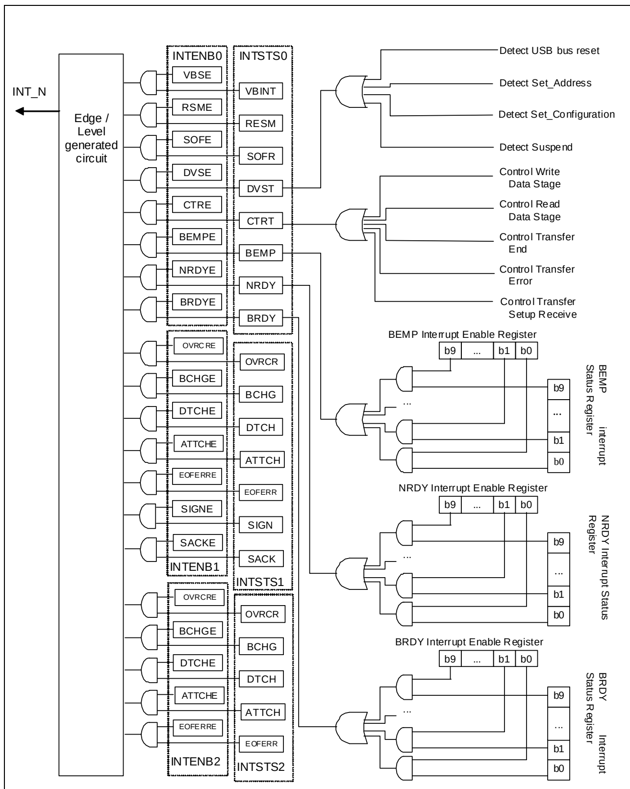
Figure 3.6 Interrupt Configuration Diagram
