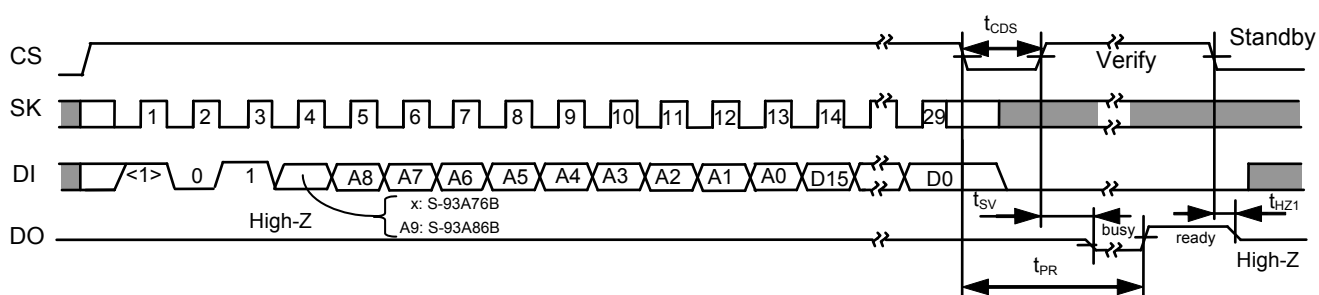
Figure 7 Data Write Timing (S-93A76B/86B)
