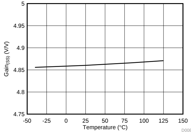
Figure 7. \text{GAIN}_{(SS)} vs Temperature
