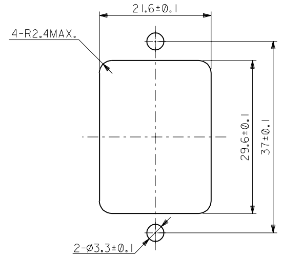
推奨パネル切り取り寸法 (後面取り付け) RECOMMENDED PANEL OPENING (REAR MOUNTING)
