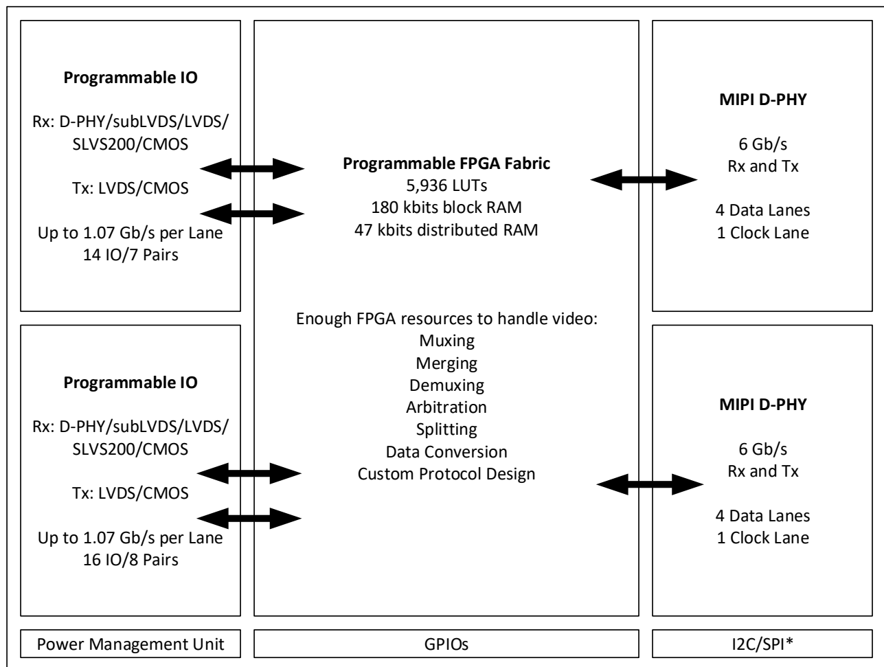
Figure 3.1. CrossLink Automotive Device Block Diagram
