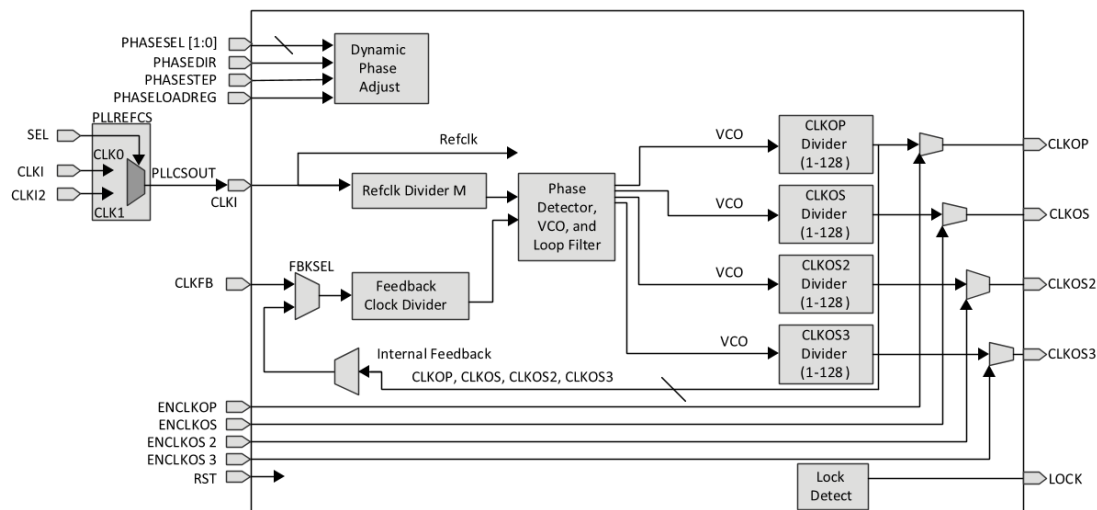
Figure 3.11. CrossLink Automotive PLL Block Diagram
