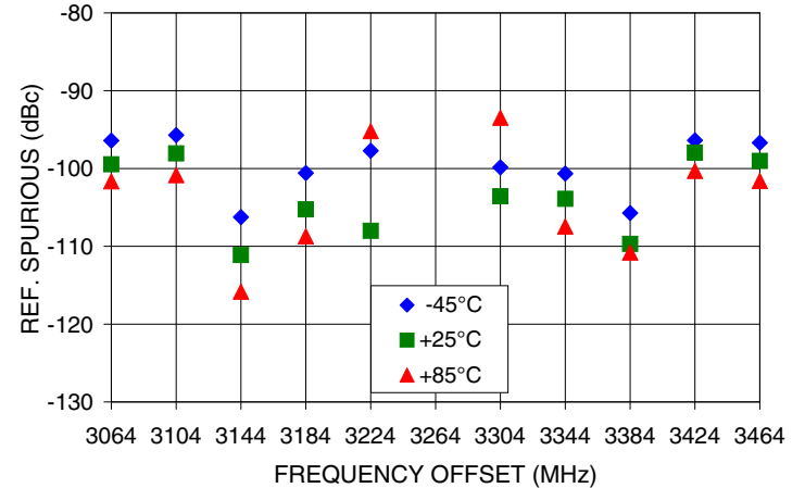
REFERENCE SPURIOUS Vs FREQ. OFFSET @ Fcar = 3264MHz
