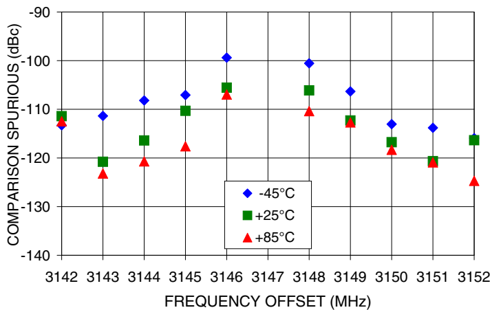
COMPARISON SPURIOUS Vs FREQ. OFFSET @ Fcar = 3147MHz
