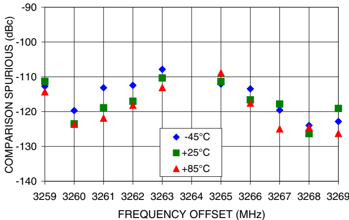
COMPARISON SPURIOUS Vs FREQ. OFFSET @ Fcar = 3264MHz
