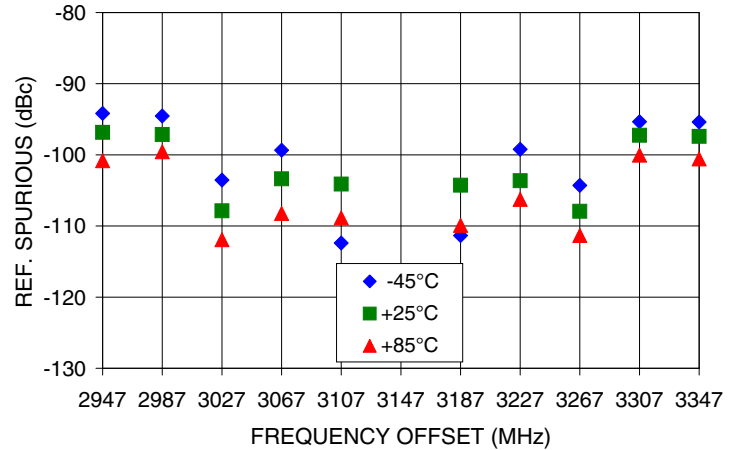
REFERENCE SPURIOUS Vs FREQ. OFFSET @ Fcar = 3147MHz
