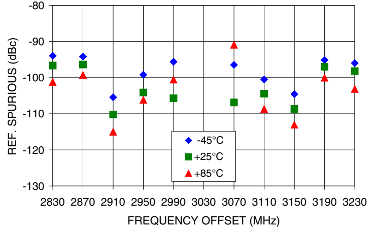
REFERENCE SPURIOUS Vs FREQ. OFFSET @ Fcar = 3030MHz
