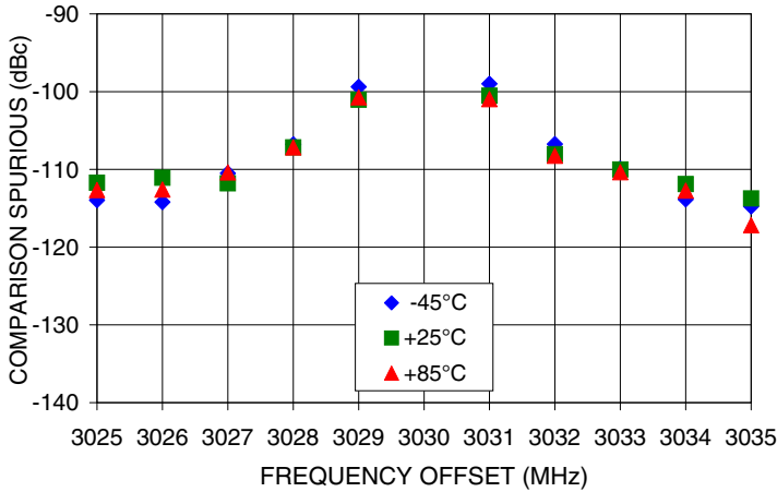
COMPARISON SPURIOUS Vs FREQ. OFFSET @ Fcar = 3030MHz
