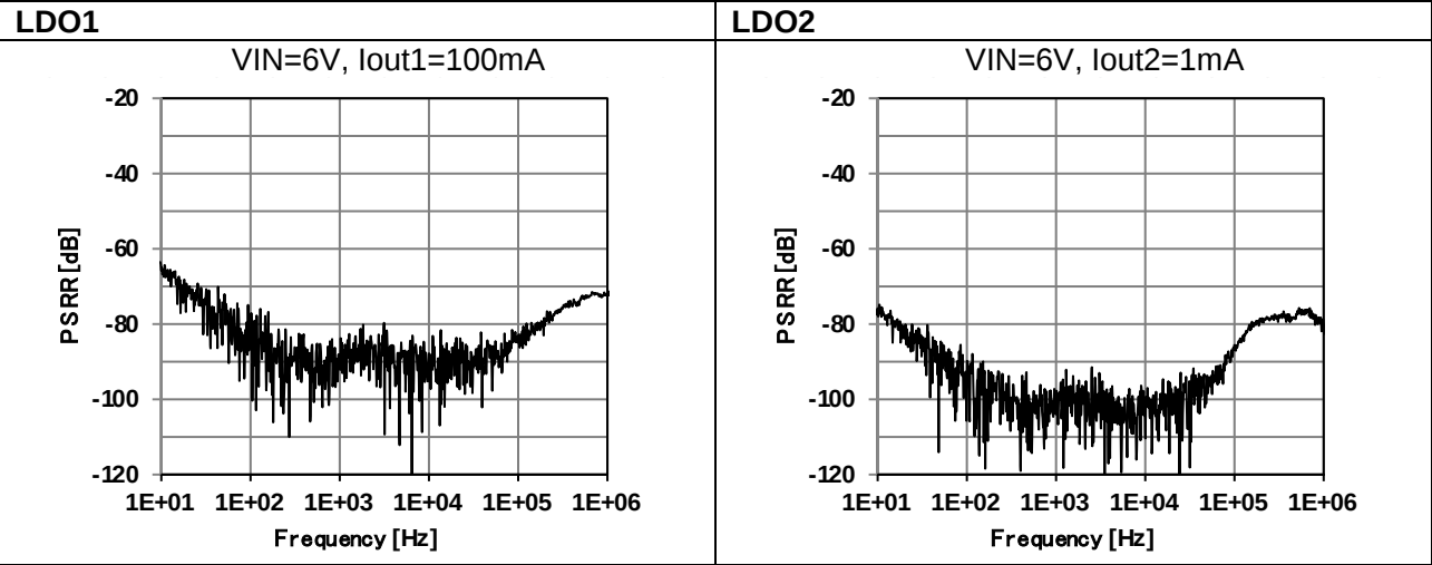
Figure 98. Ripple Rejection
