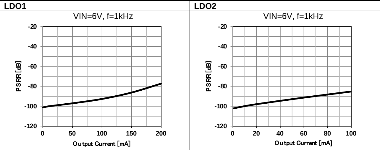
Figure 90. Ripple Rejection vs. Iout
