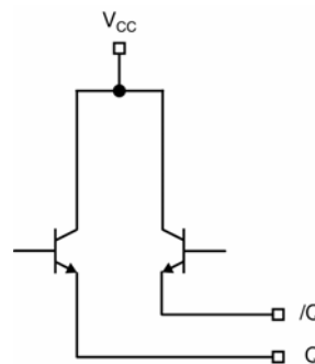
Figure 2b. Simplified LVPECL Output Stage
