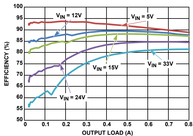
FIGURE 9. EFFICIENCY vs LOAD, PFM, V_{OUT} = 3.3\text{V}
