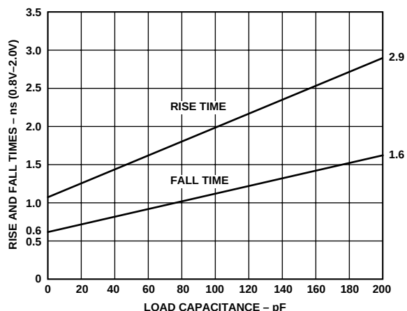
Figure 31. Typical Output Rise Time (0.8 V–2.0 V) vs. Load Capacitance ( V_{DD} = 5 V)
