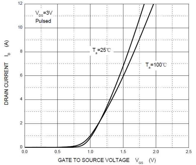
Transfer Characteristics
