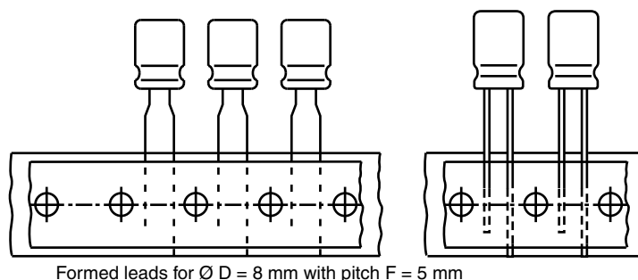
Formed leads for \varnothing D = 8 mm with pitch F = 5 mm
