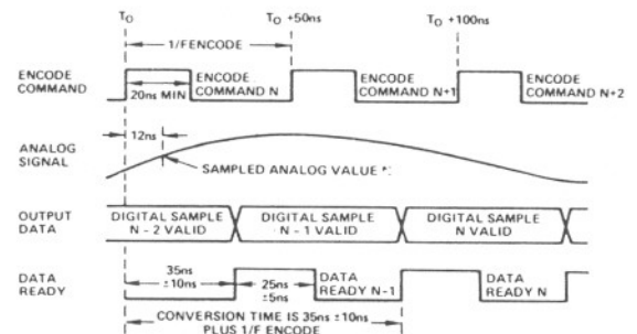
Figure 3. MATV-0820 Timing Diagram Shown at an Encode Frequency of 20MHz
