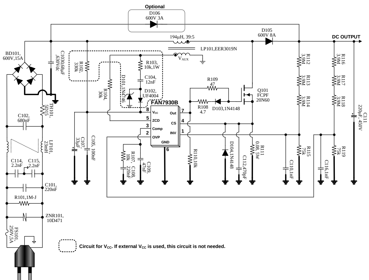
Figure 44. Demonstration Circuit
