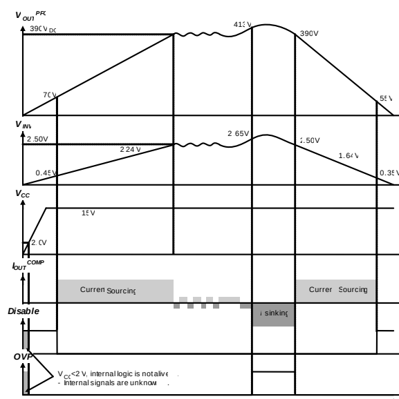
Figure 24. Timing Chart for INV Block
