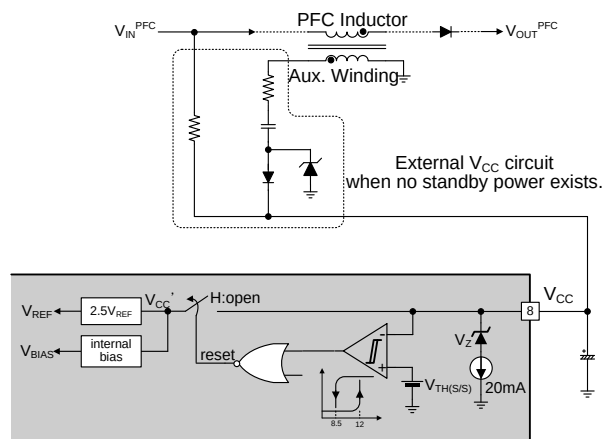
Figure 22. Startup Circuit
