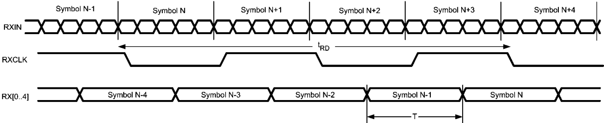
FIGURE 3. Receiver (LVDS Interface) Propagation Delay
