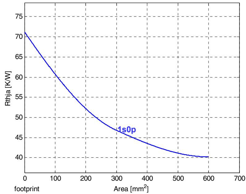
Figure 7 Typical Thermal Impedance. PCB set up 1s0p
