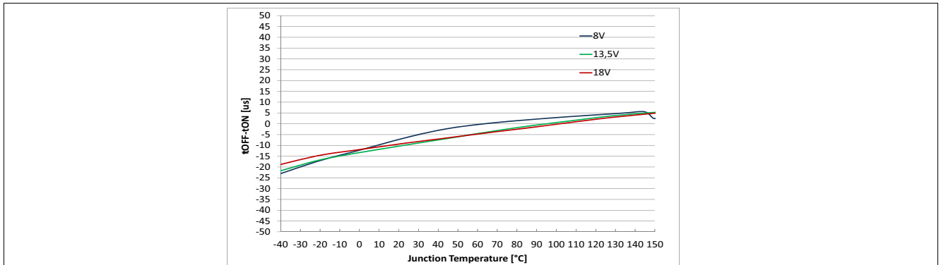
Figure 40 Turn ON / OFF matching \Delta t_{\text{SW}} = f(T_J; V_S) , R_L = 4 \Omega
