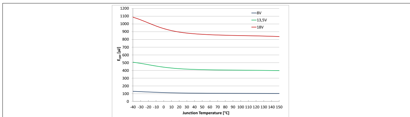
Figure 42 Switch OFF Energy E_{OFF} = f(T_J; V_{GS}) , R_L = 4 \Omega
