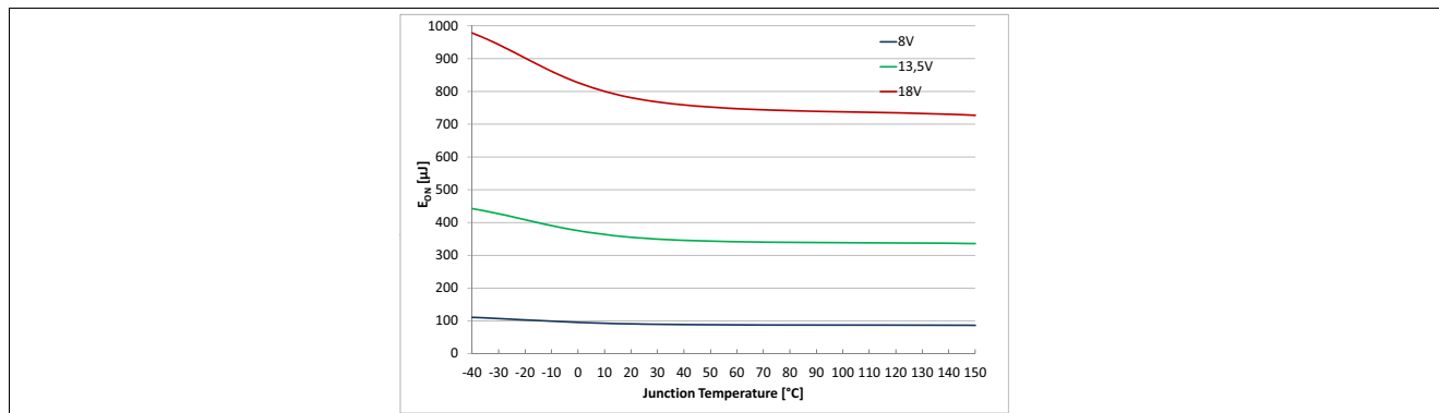
Figure 41 Switch ON Energy E_{ON} = f(T_J; V_{GS}) , R_L = 4 \Omega
