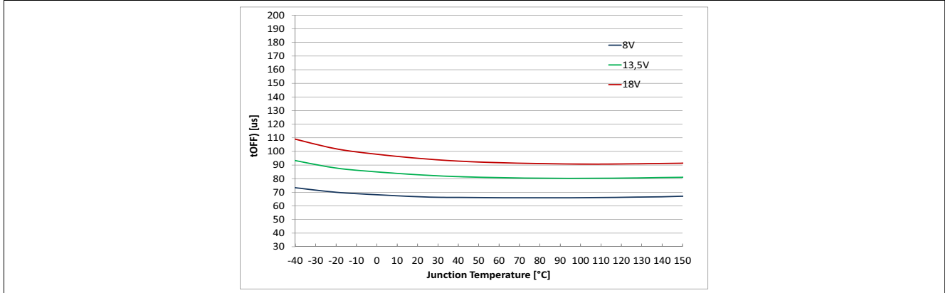
Figure 39 Turn OFF t_{\text{OFF}} = f(T_J; V_S) , R_L = 4 \Omega
