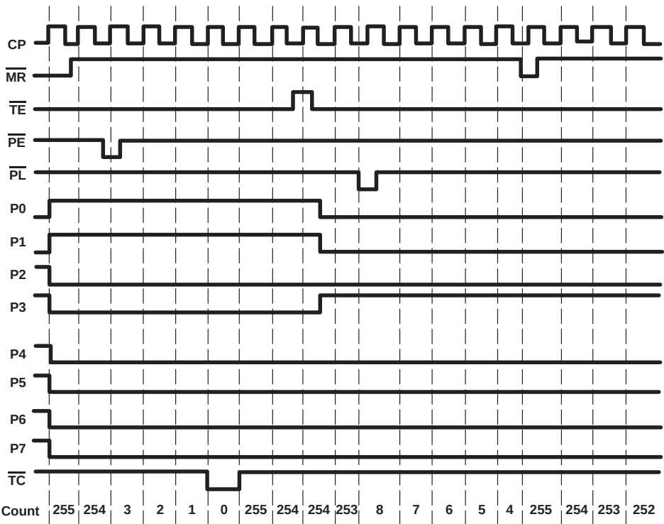
Figure 2. Timing Diagram
