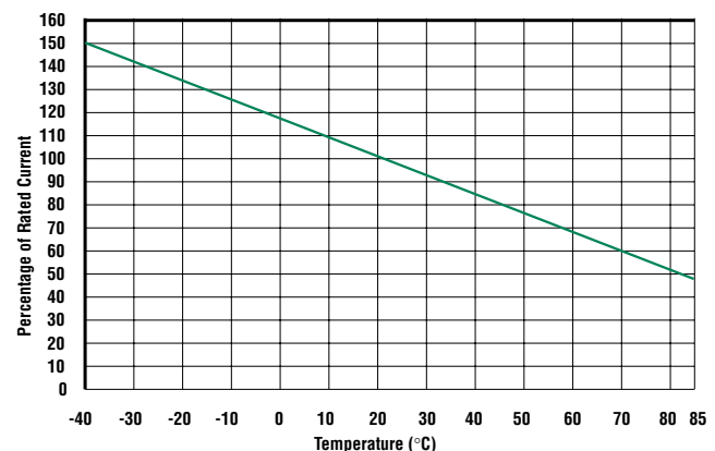
Derating Curve for 3425L Series
