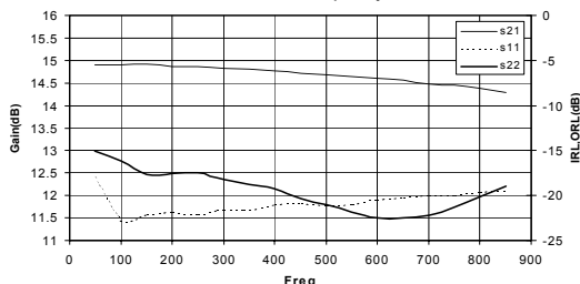
S-Parameters vs Frequency +25c
