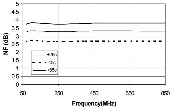
Noise Figure vs Temp
