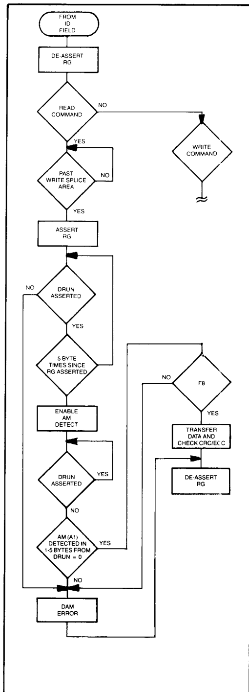
FIGURE 4. (CONT.) PPL CONTROL SEQUENCE FOR DATA FIELD
