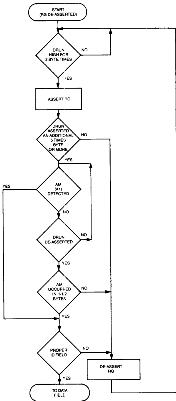
FIGURE 4. PLL CONTROL SEQUENCE FOR ID FIELD
