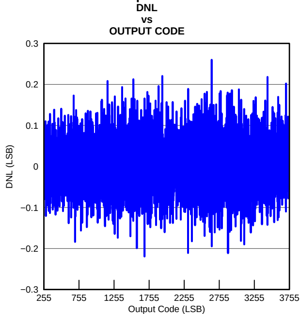
Figure 7-16. DNL Plot
