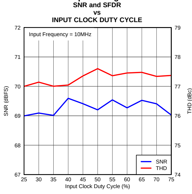
Figure 7-15. Performance Across Input Clock Duty Cycle
