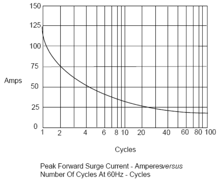
Figure 4 Maximum Non-Repetitive Forward Surge Current
