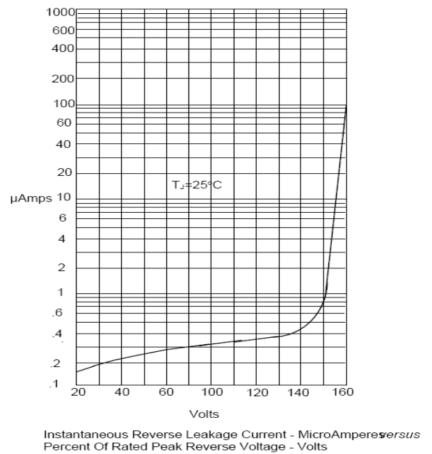
Figure 2 Typical Reverse Characteristics
