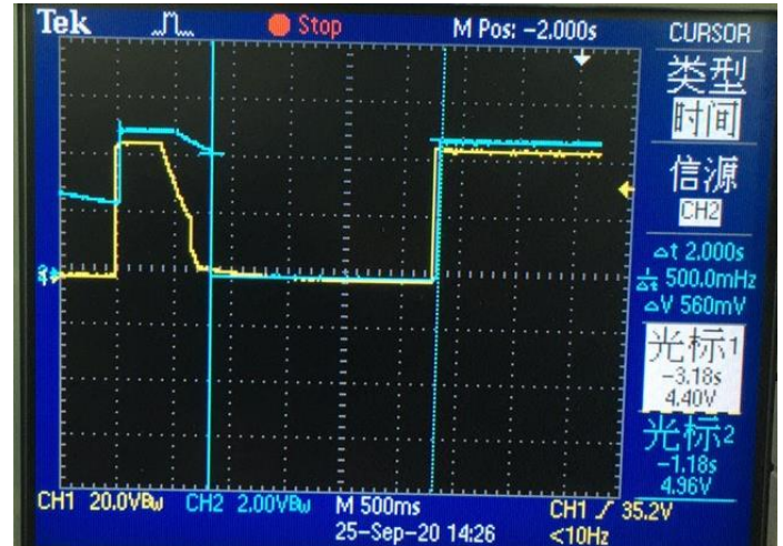
PoE switching waveform
