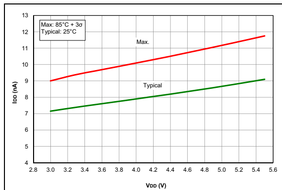
FIGURE 35-40: IPD, Brown-out Reset (BOR), BORV = 1, PIC16F1713/6 Only.
