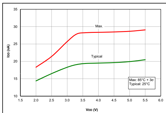
FIGURE 35-38: IPD, Fixed Voltage Reference (FVR), PIC16F1713/6 Only.
