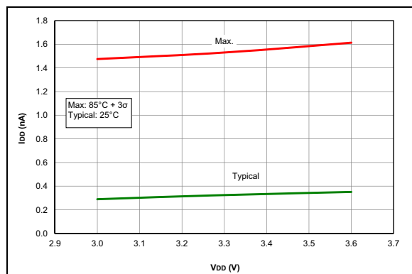
FIGURE 35-41: IPD, LP Brown-out Reset (LPBOR = 0), PIC16LF1713/6 Only.
