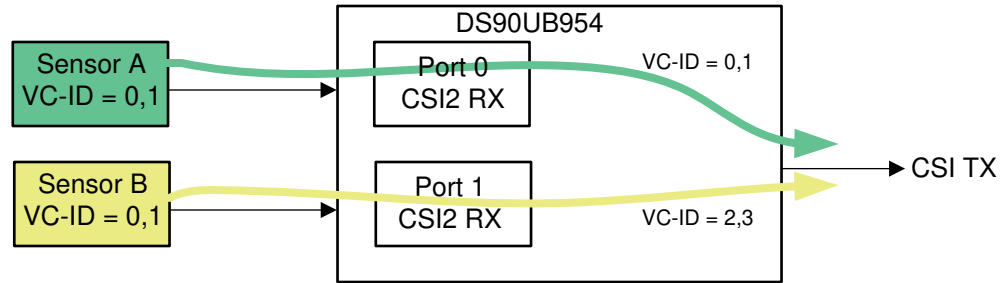
图 7-13. VC-ID Mapping Example 2
