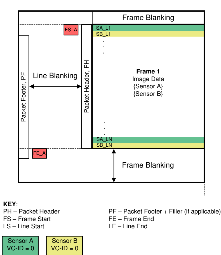
图 7-22. Line-Interleave Format
