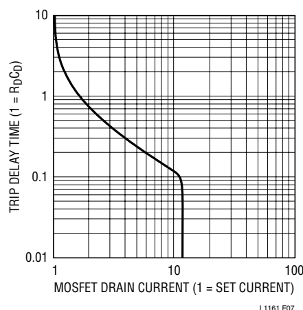
Figure 7. Current Limit Delay Time
